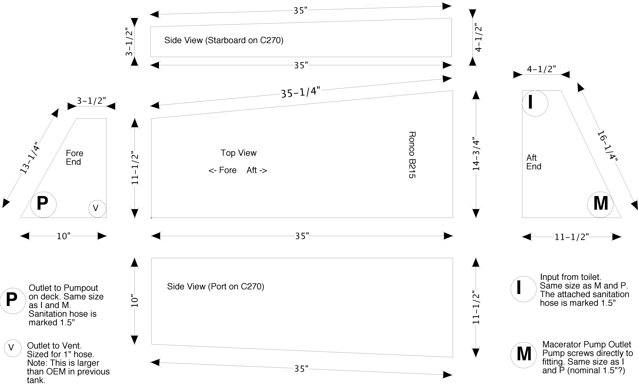
2000 Catalina 270 Holding Tank Measurements - Jyri J. Virkki - 2016
